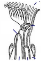
Bryozoa (1)
