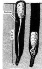
Brachiopoda
